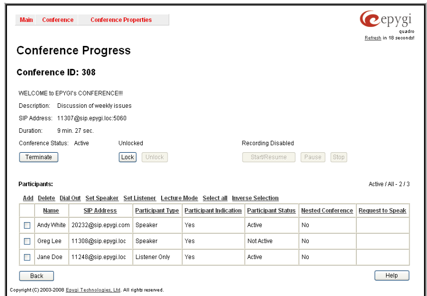
Fig. II-4: Conference Progress Page
