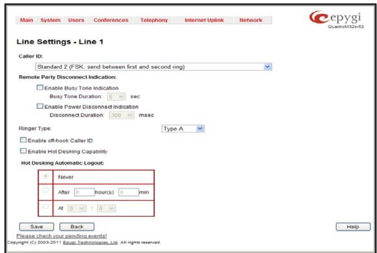
Fig. II-177: Line Codec and Caller ID Settings page
