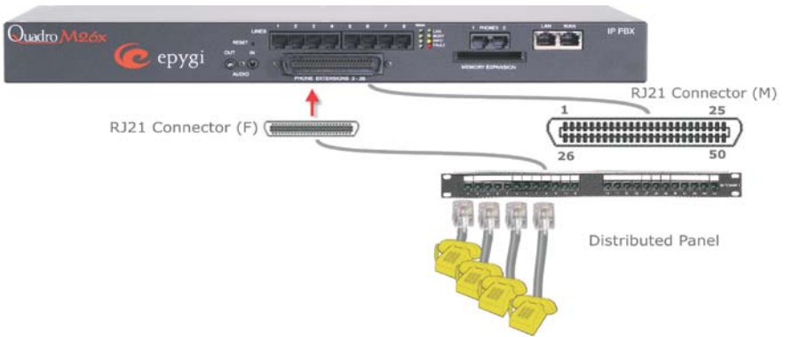
Fig. I-25: Installation: QuadroM26x connected via RJ21 connectors
