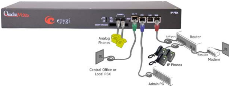
Fig. I-16: Installation: QuadroM32x behind a router with IP phones on WAN
