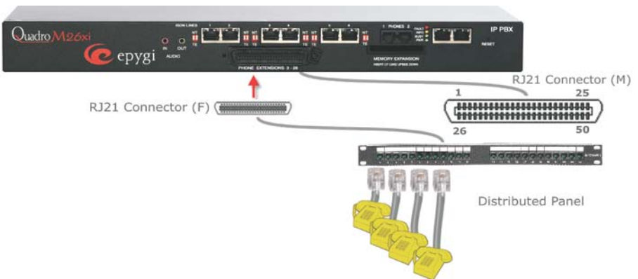
Fig. I-26: Installation: QuadroM26xi connected via RJ21 connectors
