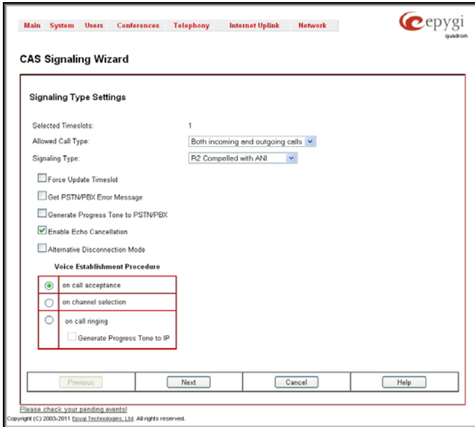
Fig. I-57: CAS Signaling Wizard - Page 1
