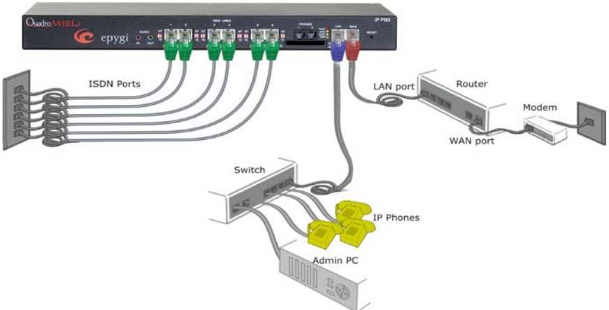
Fig. I-21: Installation: QuadroM12Li/26xi behind a router with IP phones on LAN
