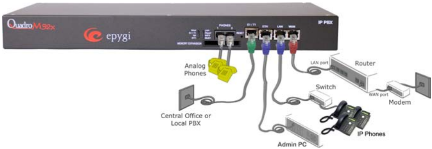
Fig. I-22: Installation: QuadroM32x used as an Internet Access Router
