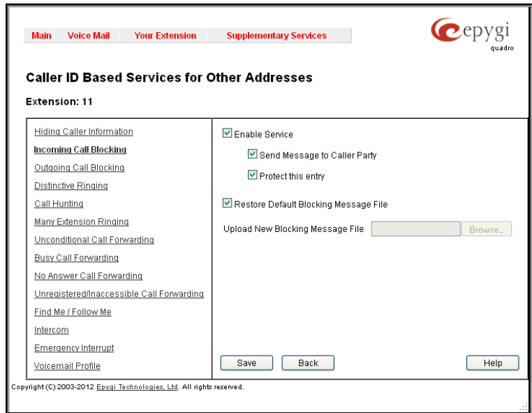
Fig. III-23 Incoming Call Blocking page
