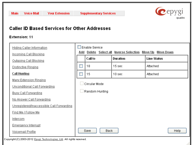
Fig. III-26 Call Hunting page
