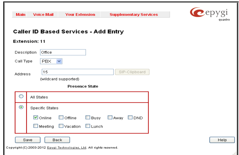
Fig.III-20 Caller ID Based Services – Add Entry page
