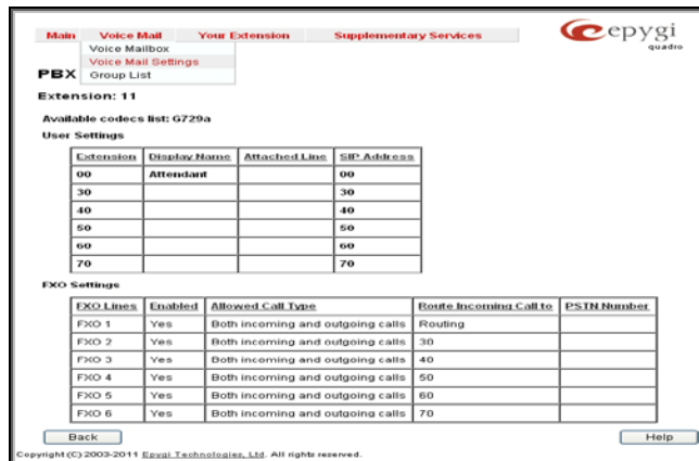
Fig. III-1 Voice Mail menu in Dynamo Theme
