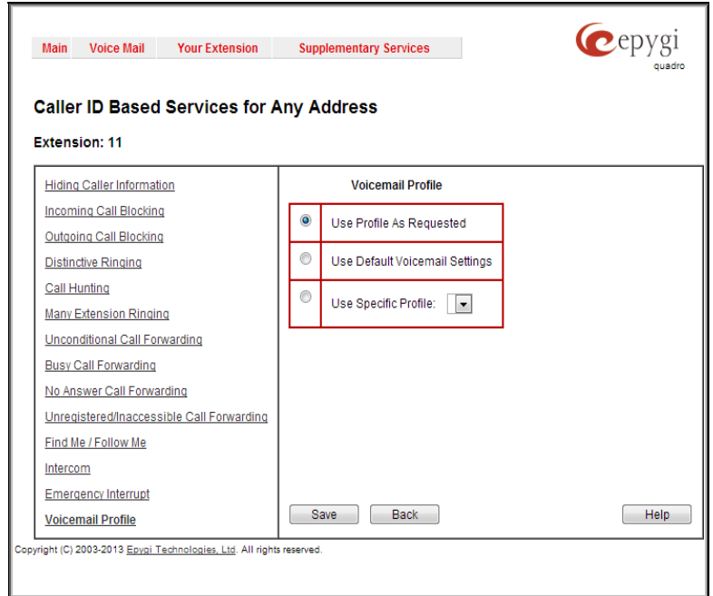
Fig. III-38 Voicemail Profile page
