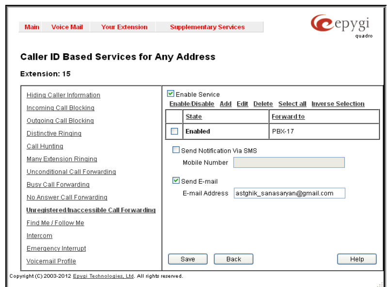
Fig. III-33 Unregistered/Inaccessible Call Forwarding page
