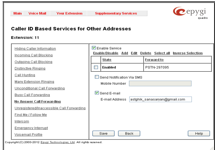
Fig. III-32 No Answer Call Forwarding page
