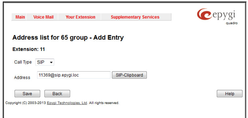
Fig. III-8 Add Address page
