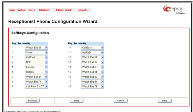
Fig. II-100: Receptionist Phone Configuration Wizard – SoftKeys Configuration for Aastra phone
